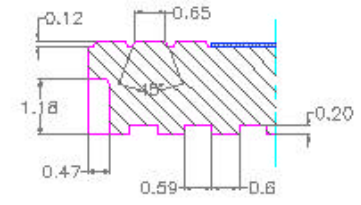
SECTION B-B SCALE 1=2
