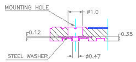
SECTION C-C SCALE 1=2
